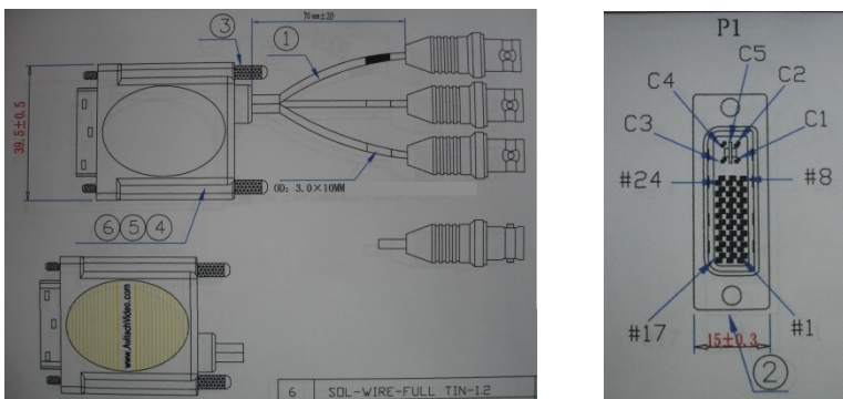
Figure 38: YPbPr to DVI Adapter wiring
