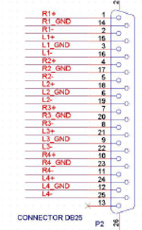
Pin-out for DB25 audio connector on Module
